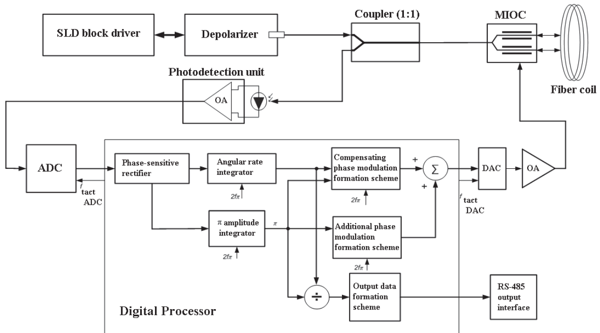
Fig. 1. FOG SRS-1000 structural scheme:
