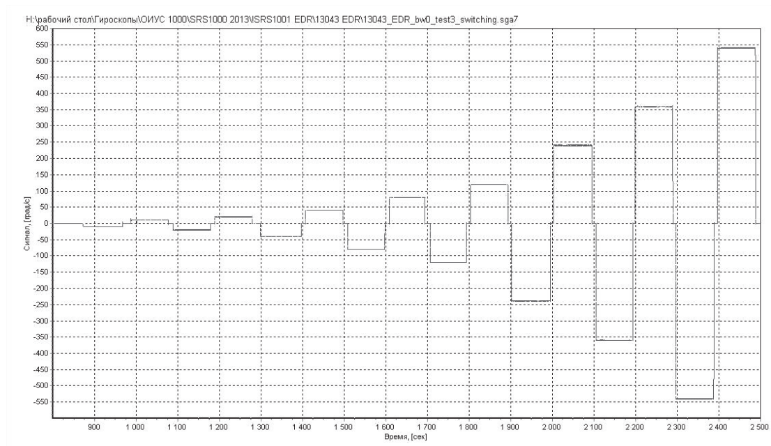
Fig. 4. SRS-1001 output signal during the stepwise angular rate change in range 10-540 ^\circ/s in single launch
