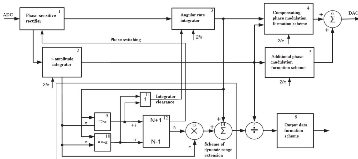
Fig. 3. FOG digital processing scheme with extended dynamic range:
