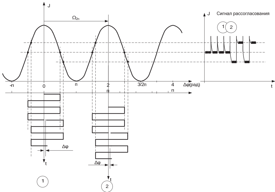
Fig. 2. Scheme of FOG output signal formation
