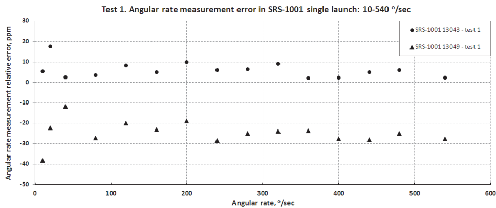
Fig. 5. Angular rate measurement relative error of two SRS-1001 devices during the stepwise angular rate change in range 10-540 ^\circ/s in single launch
