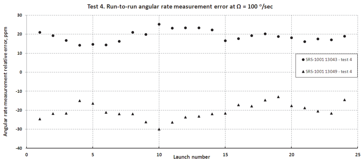
Fig. 8. SRS-1001 angular rate measurement error in tests with switching on in rotation
